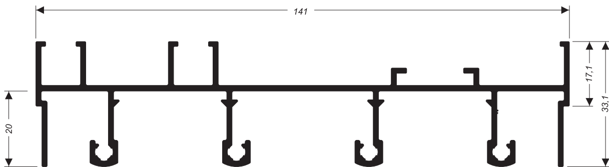
SU-121 1,586 kg/m
