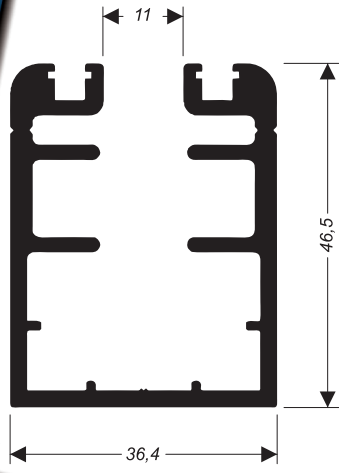
CEG-020 1,292 kg/m
