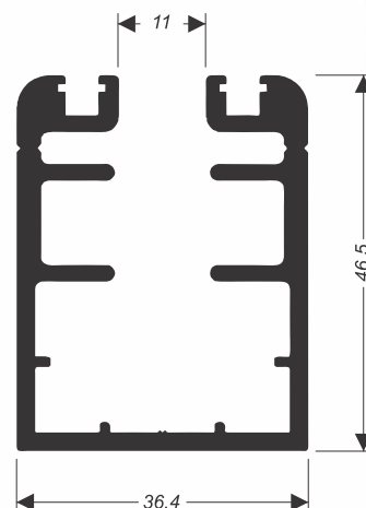
CEG-020 1,292 kg/m
